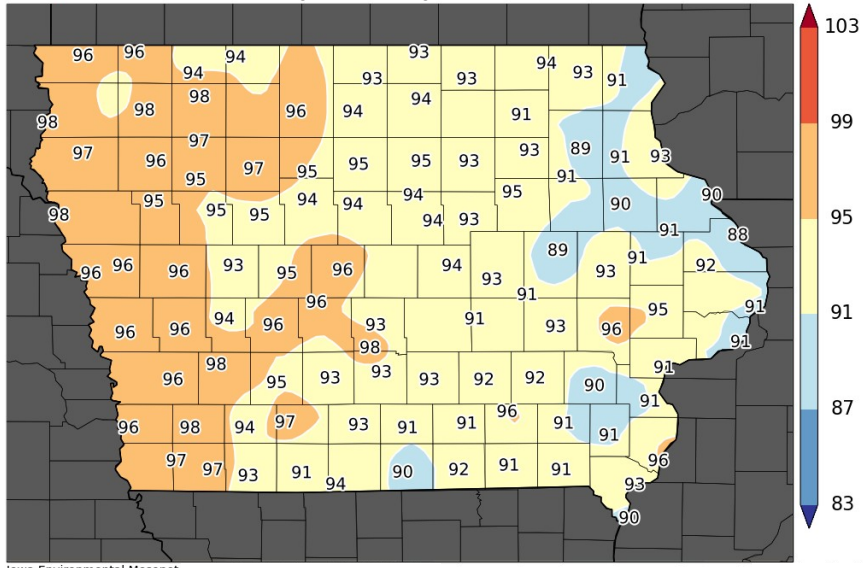
Average High Temperatures (F)
