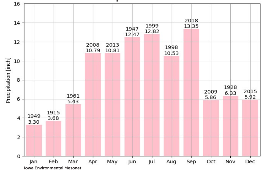
Maximum Total Monthly Precipitation [1893-2018]
